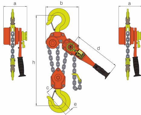
Multi Fall
